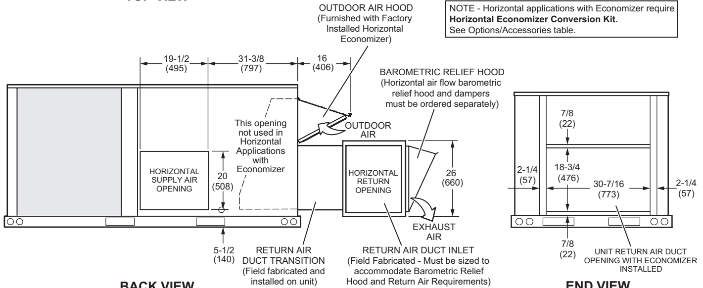
BACK VIEW
